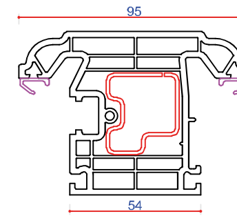
705543 (P10543) 95mm T Transom Steel Box 713158 Steel U Channel 713159 Punched Steel U 713160 35 x 30 Ported Alu 715162
