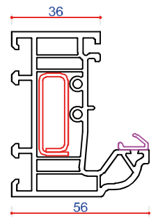
701531 (P10531) 56mm Outer Frame Steel Box 713155 Steel Box 713187 Steel U Channel 713185 Thermal Insert 709331
