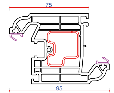
705545 (P10545) 95mm Z Transom Steel Box 713158 Steel U Channel 713159 Punched Steel U 713160
