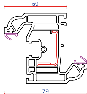
703539 (P10539) Tilt & Turn Sash Steel L Section 713161
