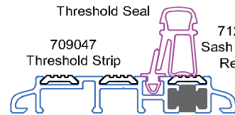
704289 (A00289) Part M Low Threshold
