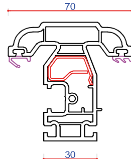
703638 (P10638) Internally Beaded Sash/Transom Steel P Section 713183 Steel P Section 713184 13 x 23 Ported Alu 715164
