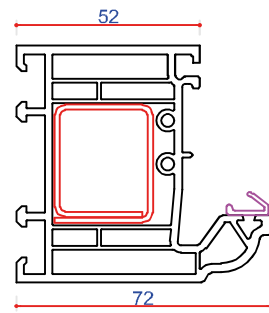
701532 (P10532) 72mm Outer Frame Steel Box 713174 Steel Box 713191 Steel U Channel 713186 Steel P Section 713157 Thermal Insert 709332
