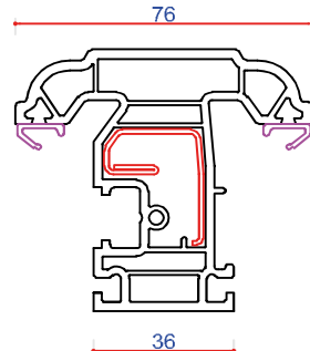
703538 (P10538) Internally Beaded Sash Steel P Section 713152
