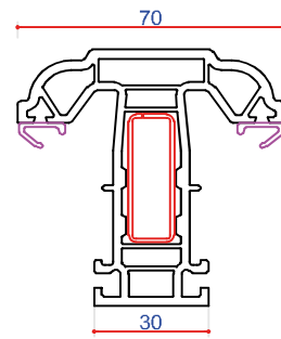
702533 (P10533) 70mm T Transom Steel Box 713187 Steel Box 713155 35 x 12.5 Ported Alu 715161
