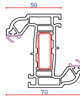
702536 (P10536) 70mm Z Transom Steel Box 713187 Steel Box 713155
