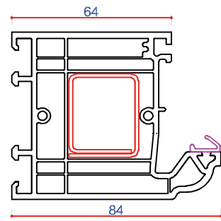
701204 84mm Outer Frame Steel Box 713174 Steel Box 713191 Steel U Channel 713186 Steel P Section 713157 Thermal Insert 709332
