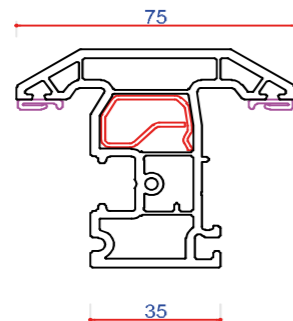
703508 (P10508) Internally Beaded Sash Steel P Section 713182
