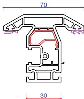
703514 (P10514) Internally Beaded Sash / Transom Steel P Section 713183 Steel P Section 713184
