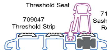
704289 (A00289) Part M Low Threshold
