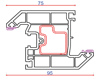
705515 (P10515) 95mm Z Transom Steel Box 713158
