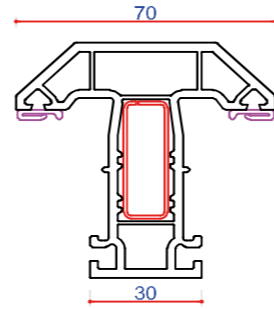
702503 (P10503) 70mm T Transom Steel Box 713187 Steel Box 713155 35 x 12.5 Ported Alu 715161
