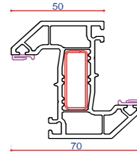
702506 (P10506) 70mm Z Transom Steel Box 713187 Steel Box 713155
