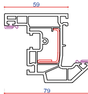
703509 (P10509) Tilt & Turn Sash Steel L Section 713161
