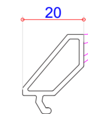
107154 28mm Bevelled Glazing Bead
