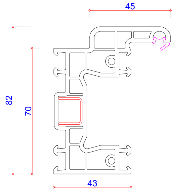
105174 65mm Outer Frame Steel U Channel 113391
