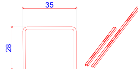
113393-900001 Sash (Prepped) Reinforcement (Main/French/2-2)
