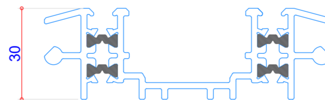
104392 Low Threshold (Champagne Only)
