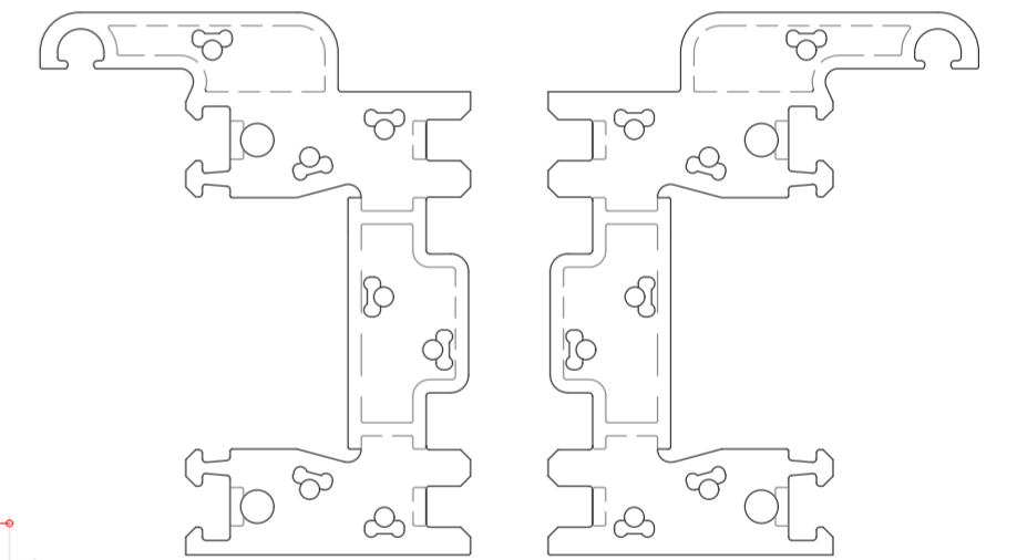
109998 Thermally Broken Threshold Mechanical Joint
